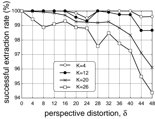
Figure 5. Extraction accuracy of cross ratios.
